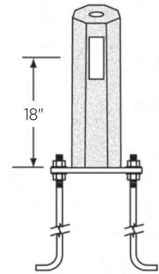
Elevation See recommended "capping details"
